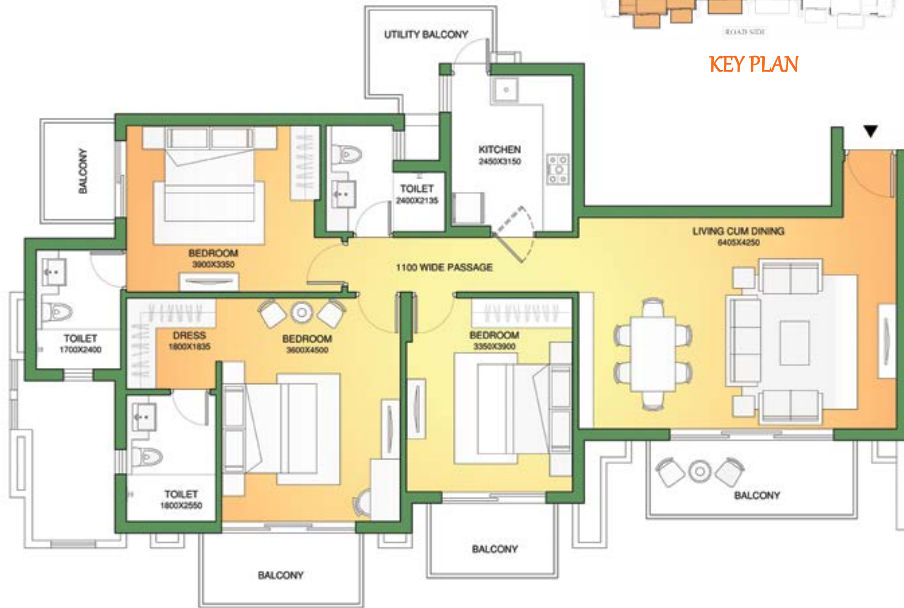
FLOOR PLAN
